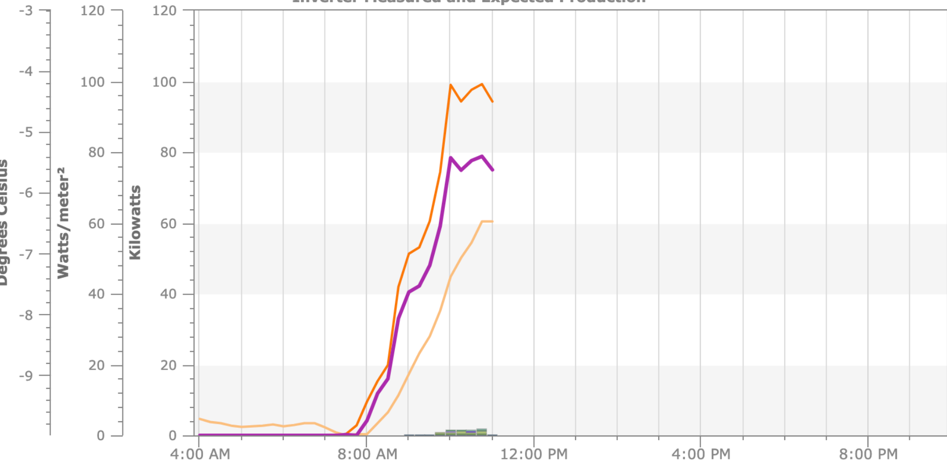
Inverter Measured and Expected Production
